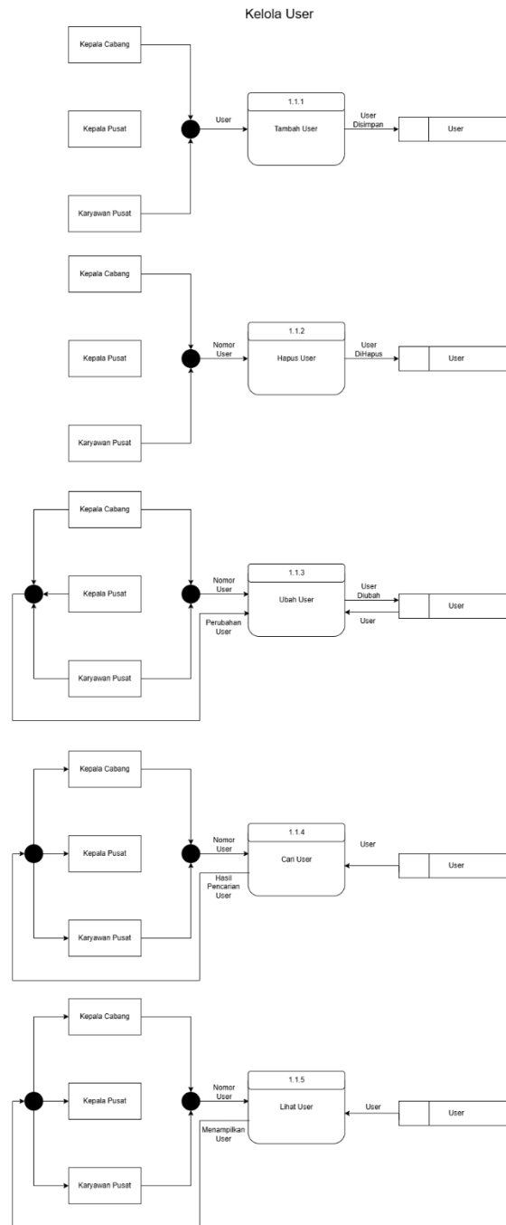
Gambar 4.34 Data Flow Diagram User
