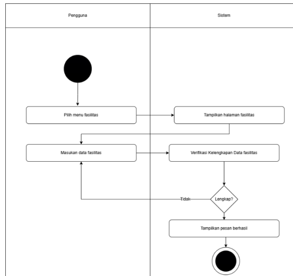
Gambar 1.22 Activity Diagram Tambah Fasilitas
