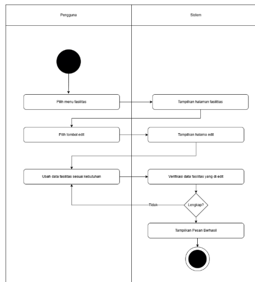
Gambar 1.23 Activity Diagram Ubah Fasilitas
