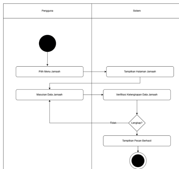
Gambar 1.18 Activity Diagram Tambah Jamaah
