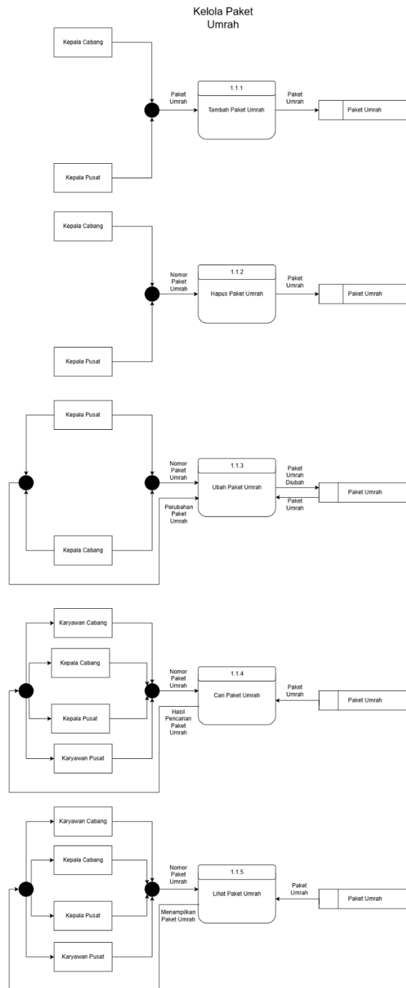
Gambar 4.31 Data Flow Diagram Paket
