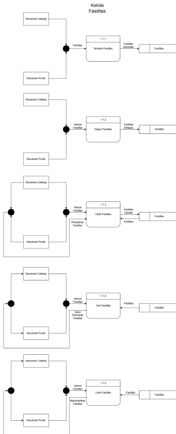
Gambar 4.30 Data Flow Diagram Fasilitas
