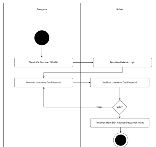
Gambar 1.1 Activity Diagram Login
