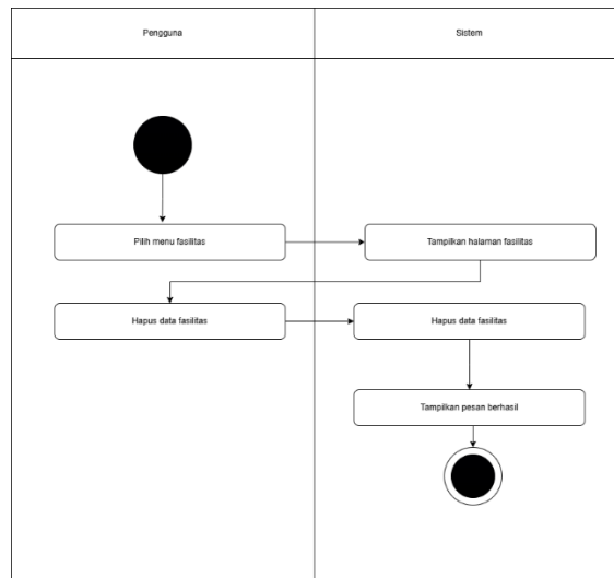
Gambar 1.24 Activity Diagram Hapus Fasilitas
