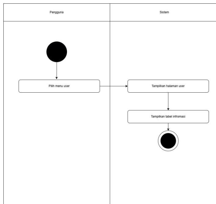
Gambar 1.5 Activity Diagram Lihat User
