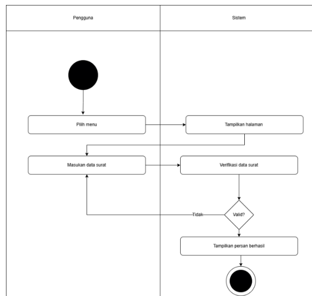
Gambar 1.6 Activity Diagram Tambah Surat
