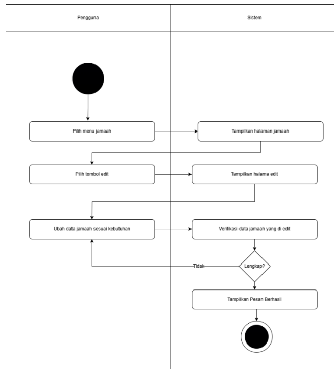
Gambar 1.19 Activity Diagram Ubah Jamaah
