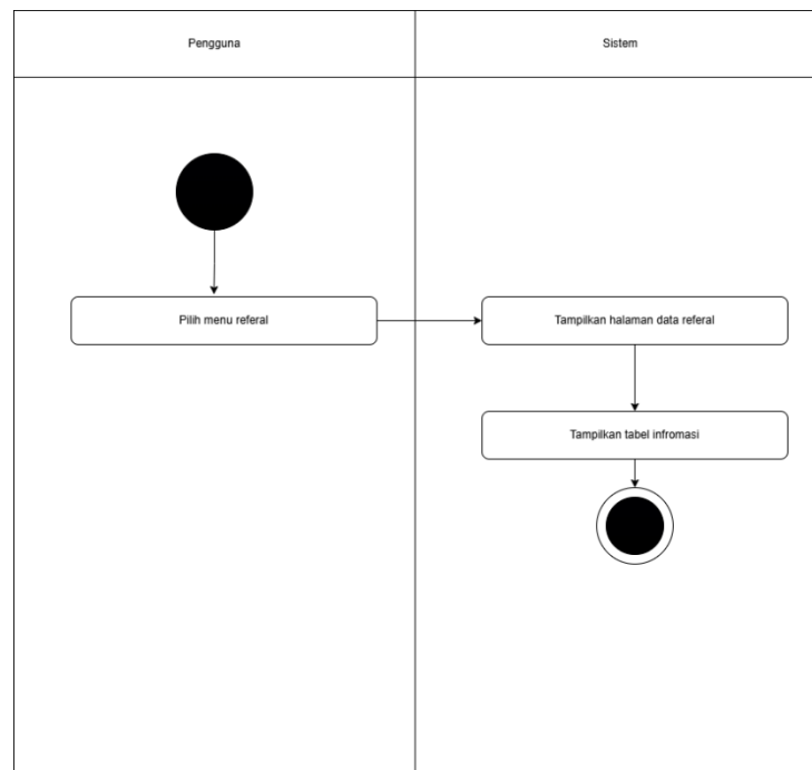
Gambar 1.26 Activity Diagram Lihat Referrals
