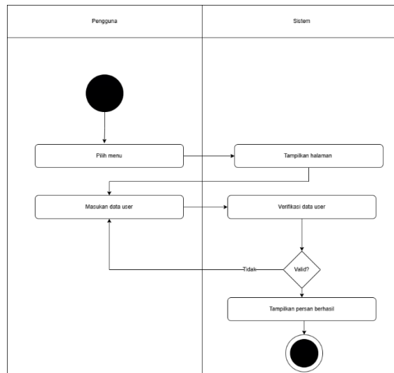
Gambar 1.2 Activity Diagram Tambah User
