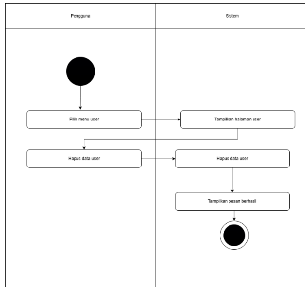
Gambar 1.4 Activity Diagram Hapus User
