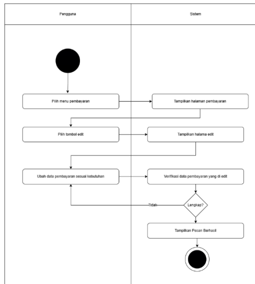
Gambar 1.11 Activity Diagram Ubah Pembayaran
