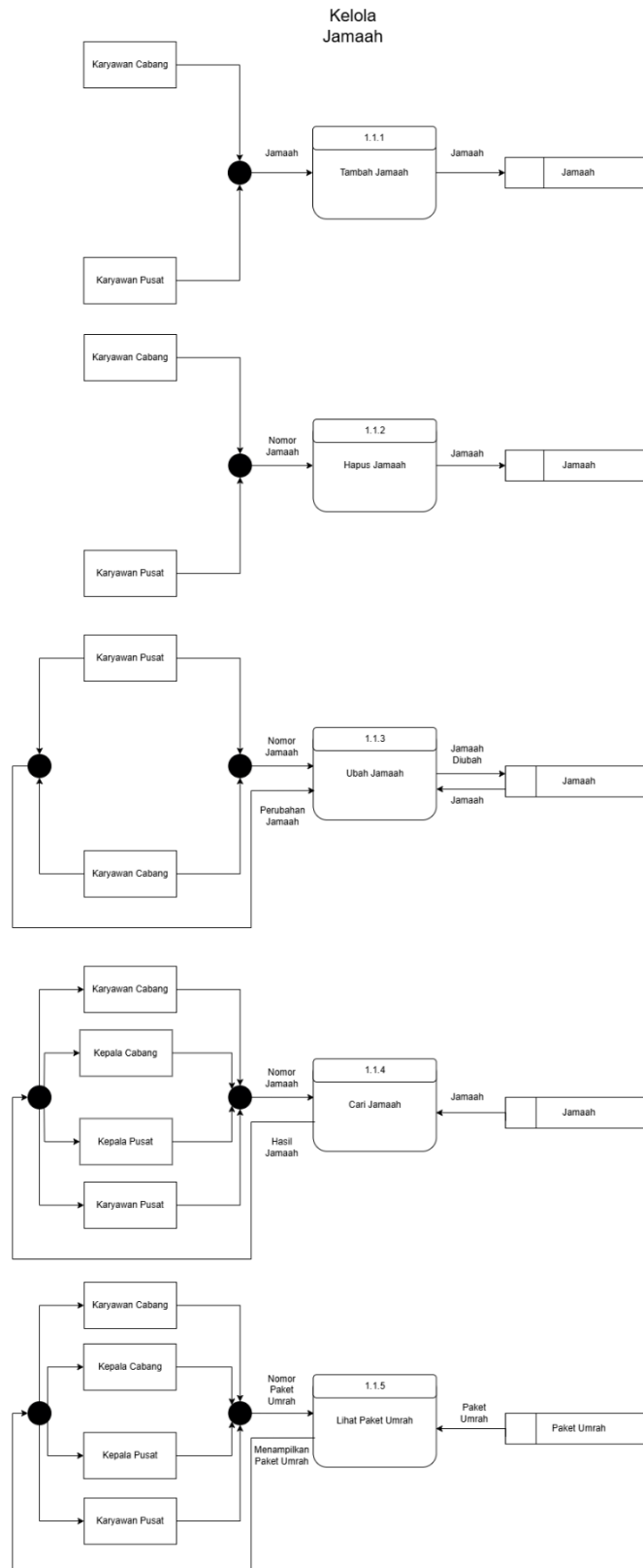
Gambar 4.29 Data Flow Diagram jamaah
